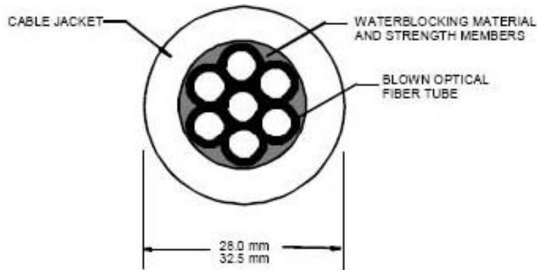
FIGURE 2. Seven-tube cable.
